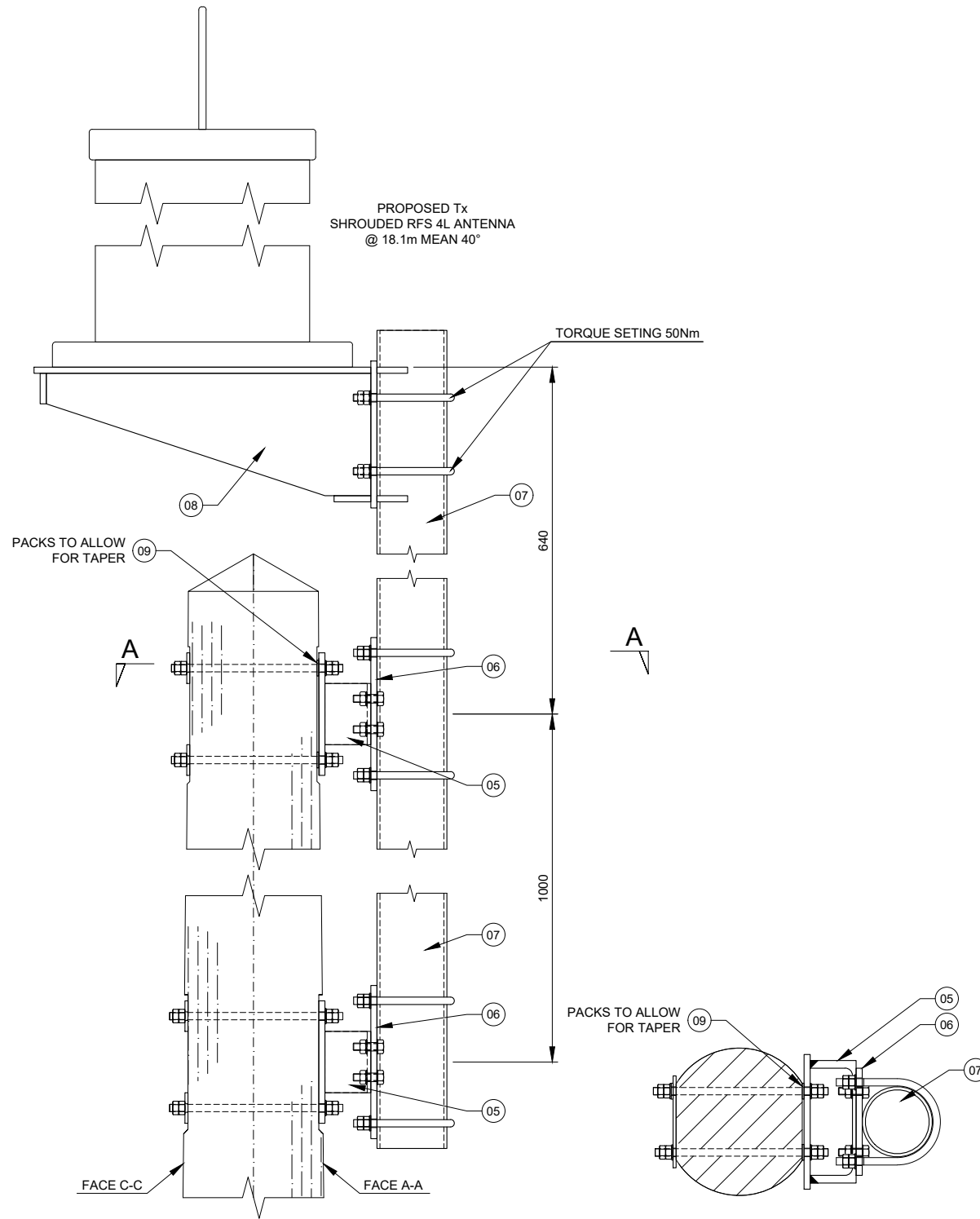
DETAIL F - Tx ANTENNA MOUNT Scale 1:10
