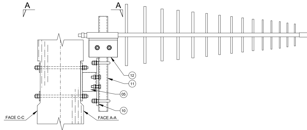
DETAIL G - Rx ANTENNA MOUNT Scale 1:10
