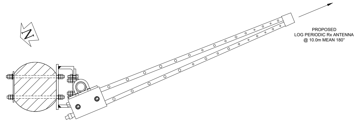
VIEW A-A Scale 1:10
